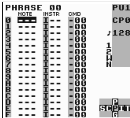
Figure 1.3: Phrase Screen
